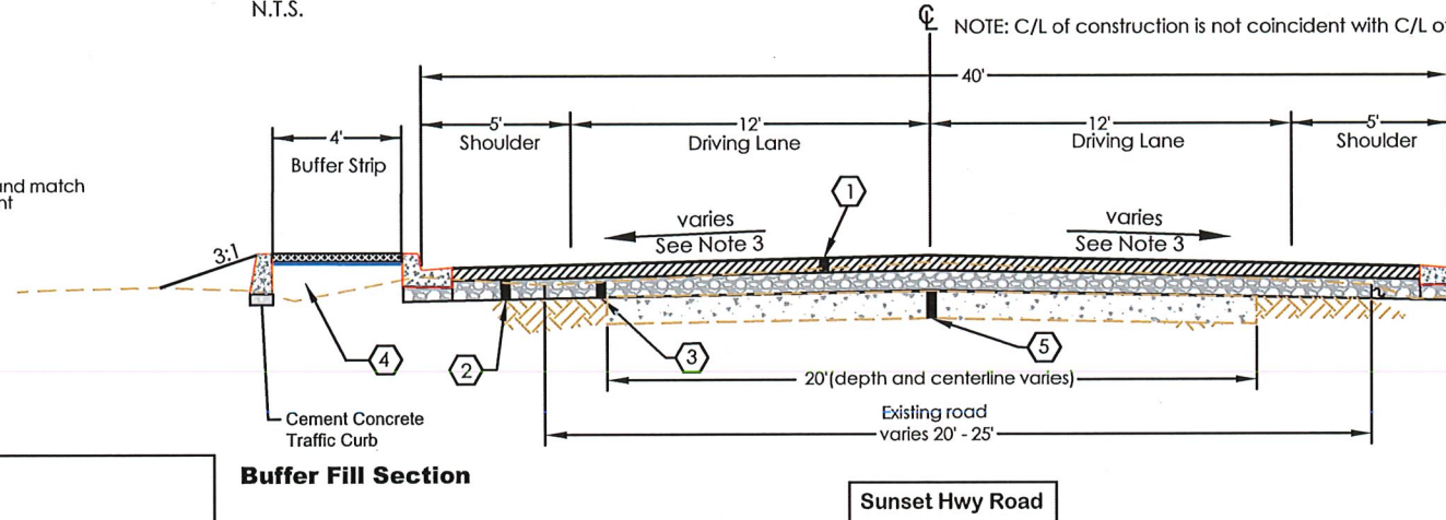
TYPICAL CITY SECTION Sunset Hwy Road Sta. S-188+52 to S-200+50 N.T.S.
