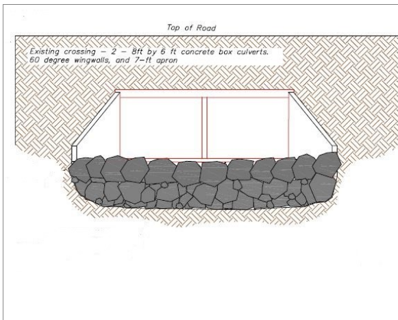
Project Typical Section
