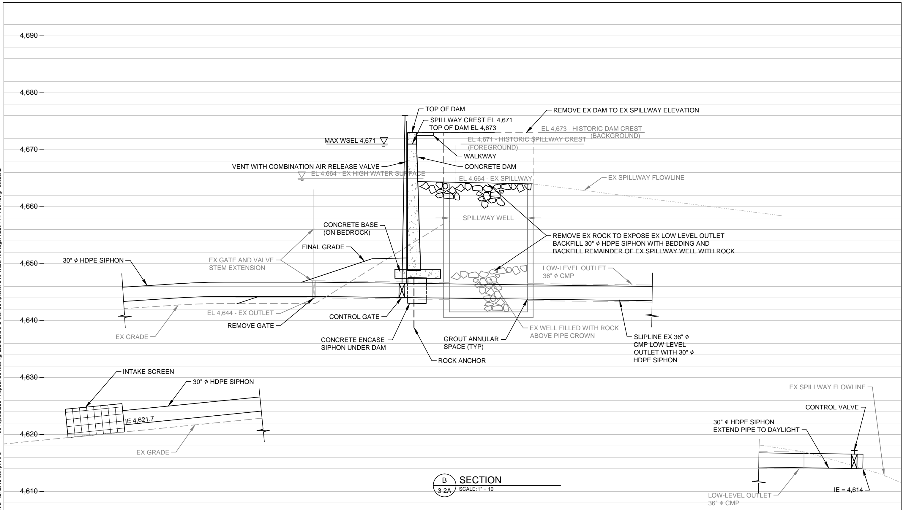
Figure 3-2B Improvement Section, Option 2 - Increase Useable Storage to 2,500 Acre-feet Appraisal Study Eightmile Lake Storage Restoration Chelan County Natural Resources Department/Icicle and Peshastin Irrigation Districts
