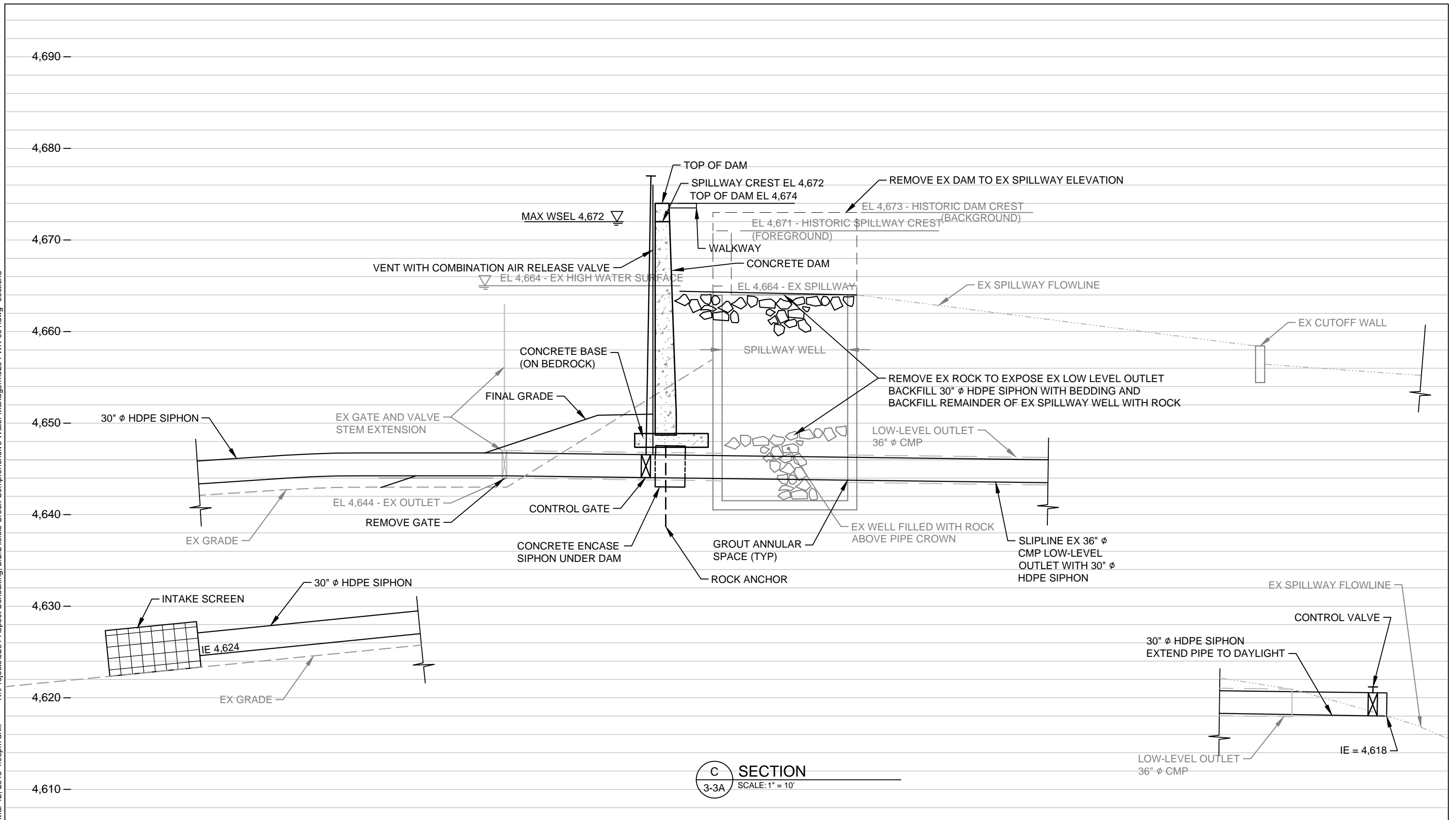
Figure 3-3B Improvement Section, Option 3 - Increase Useable Storage to 2,500 Acre-feet Appraisal Study Eightmile Lake Storage Restoration Chelan County Natural Resources Department/Icicle and Peshastin Irrigation Districts
