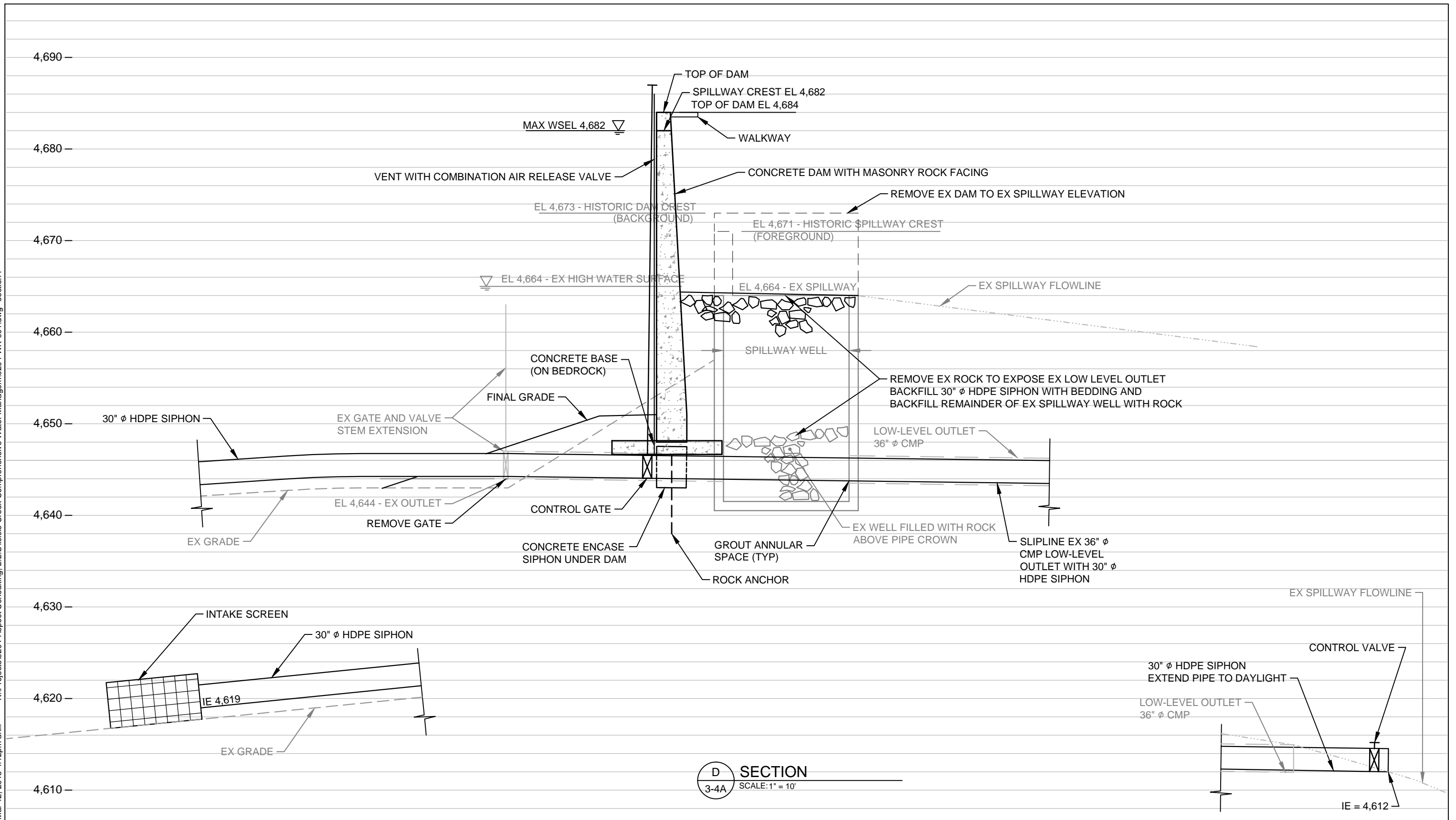
Figure 3-4B Improvement Section, Option 4 - Increase Useable Storage to 3,500 Acre-feet Appraisal Study Eightmile Lake Storage Restoration Chelan County Natural Resources Department/Icicle and Peshastin Irrigation Districts
