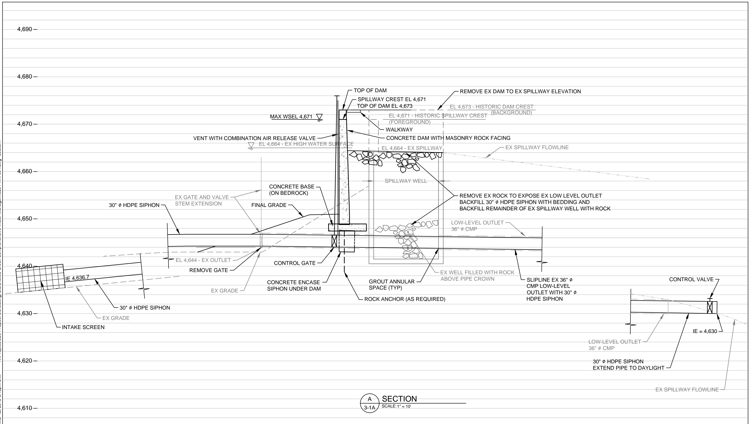
Figure 3-1B Improvement Section, Option 1 - Increase Useable Storage to 2,000 Acre-feet Appraisal Study Eightmile Lake Storage Restoration Chelan County Natural Resources Department/Icicle and Peshastin Irrigation Districts
