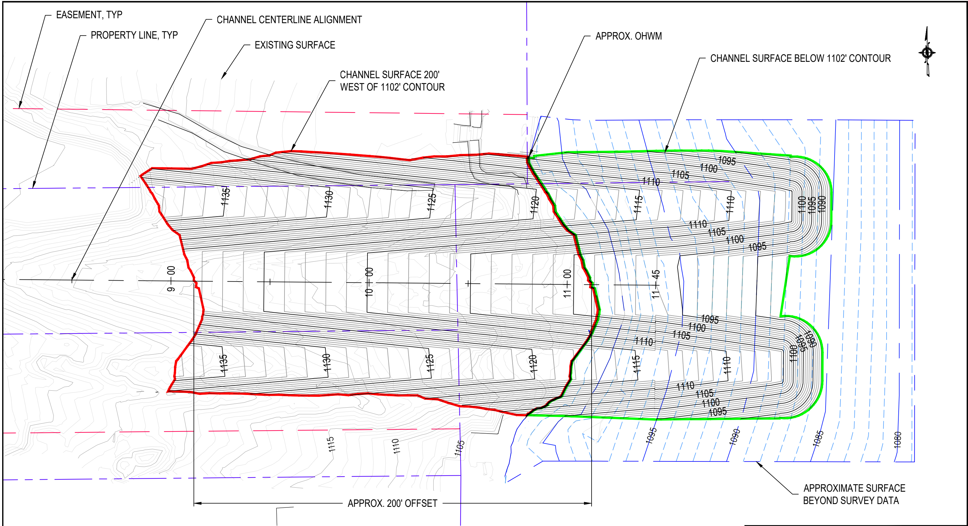
CHANNEL PLAN VIEW 1" = 30'
