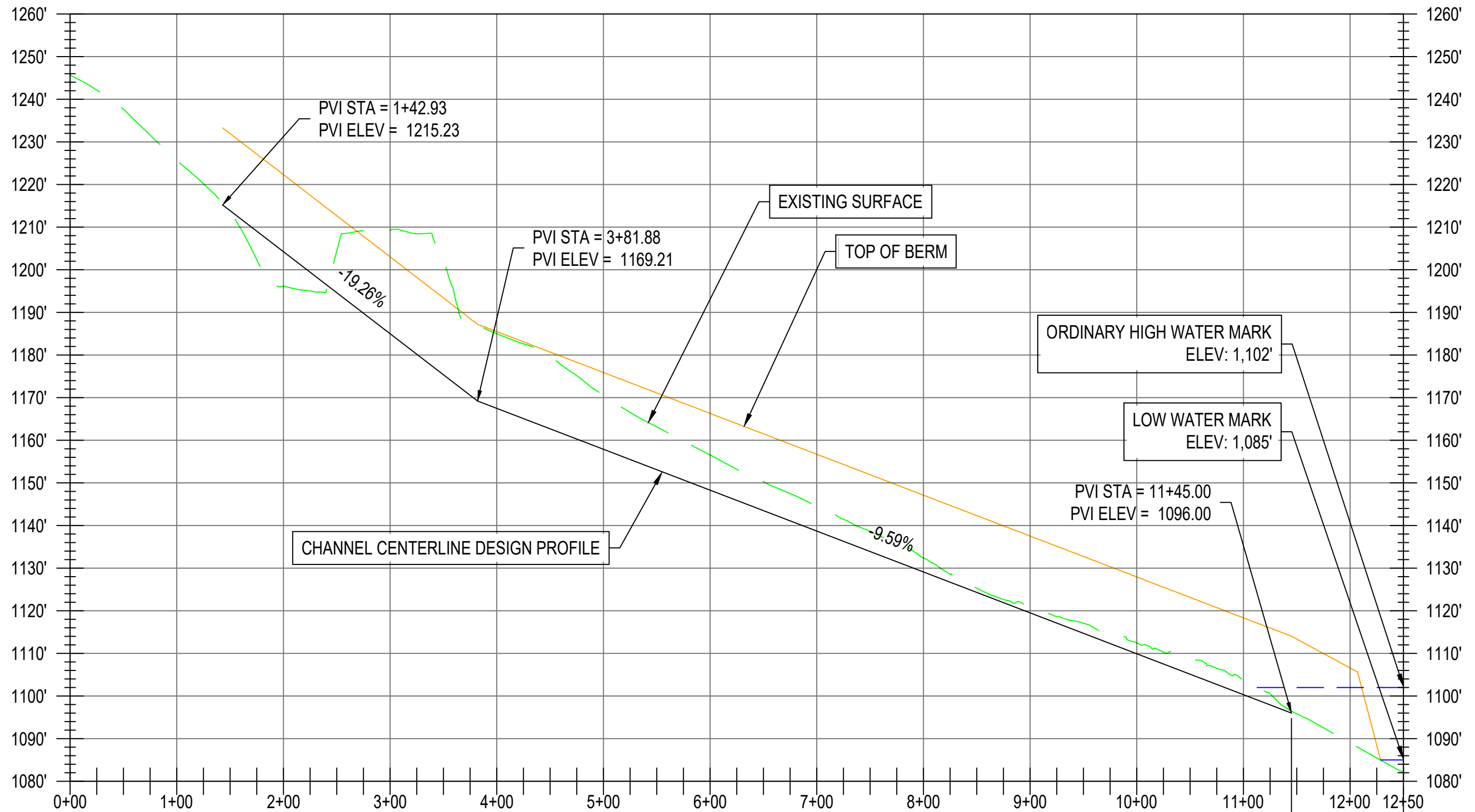
CHANNEL CENTERLINE DESIGN PROFILE
