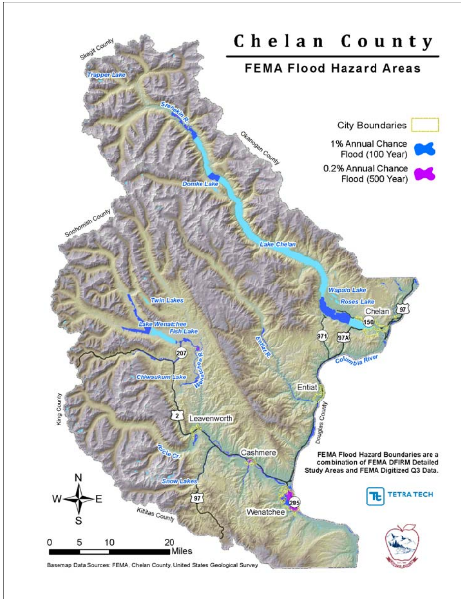
Figure 7-1. Mapped Flood Hazard Areas in Chelan County
