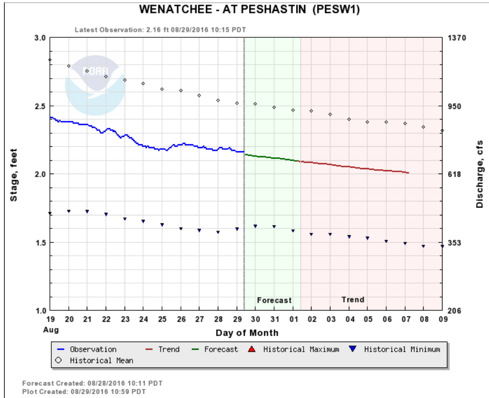
Figure 7-2. Wenatchee River Hydrograph at Peshastin
