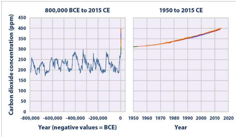
Figure 10-1. Global Carbon Dioxide Concentrations Over Time
