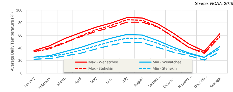
Figure 3-2. Average Daily Temperatures
