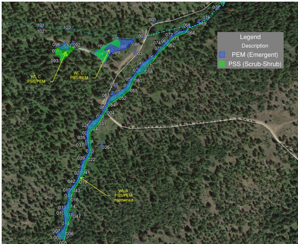
Figure A-32. Cowardin Plant Classes
