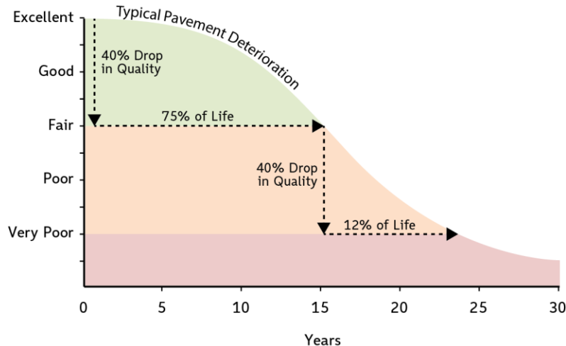
Figure 18. National Standard Deterioration Curve for Pavement
