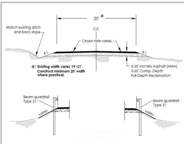
Typical Section
